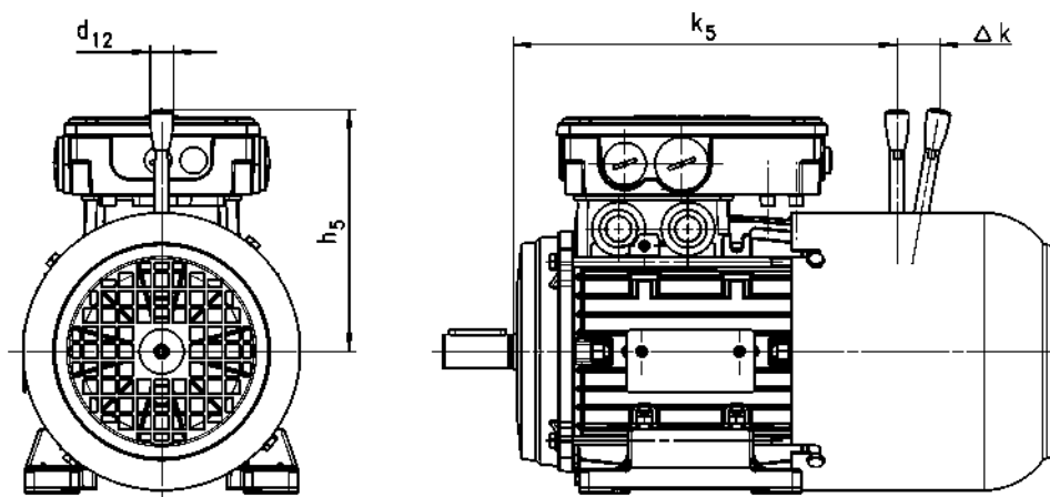
Manual release lever for IEC motors
